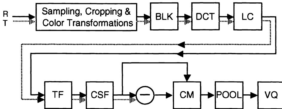
Figure 1. Overview of DVQ processing steps.
