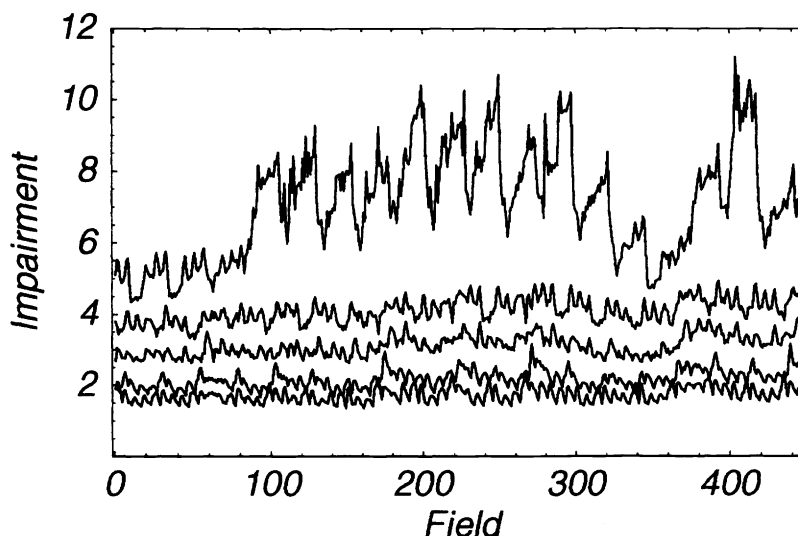
Figure 4. Impairment in each field for the source “flower” and HRC’s 1-5 (codec A at bit-rates of 2-10 Mbit/sec).
